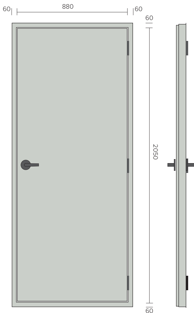
APERTURE SIZE TO SUIT DOOR Height = 2060mm Width = 890mm
