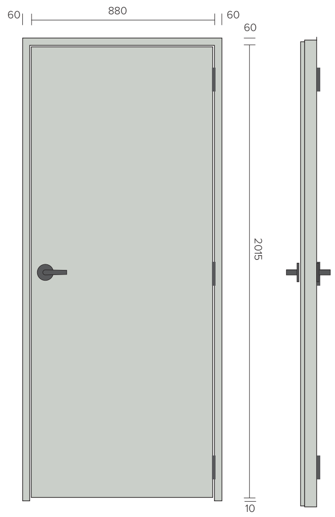
APERTURE SIZE TO SUIT DOOR Height = 2025mm Width = 890mm
