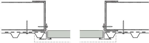
DOOR PLAN VIEW
